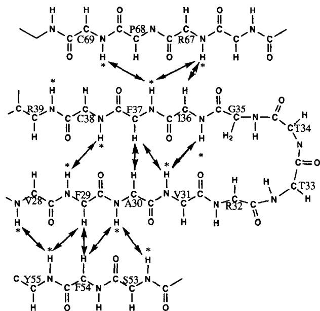
Fig. 3. Schematic diagram of the arrangement of the four-stranded \beta -sheet of the N-ada 14k fragment. Arrows indicate the observed interstrand NOE's. Amide protons with slow H-D exchange rates are indicated by asterisks.
